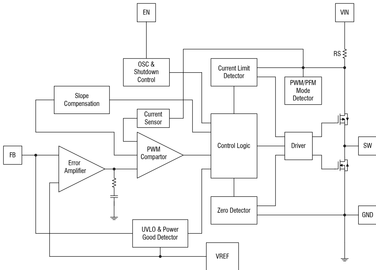
Figure 2. MT3410L Block Diagram
