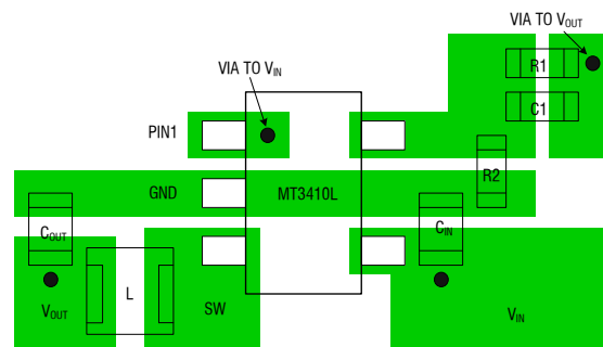
Figure 3. MT3410L Suggested Layout
