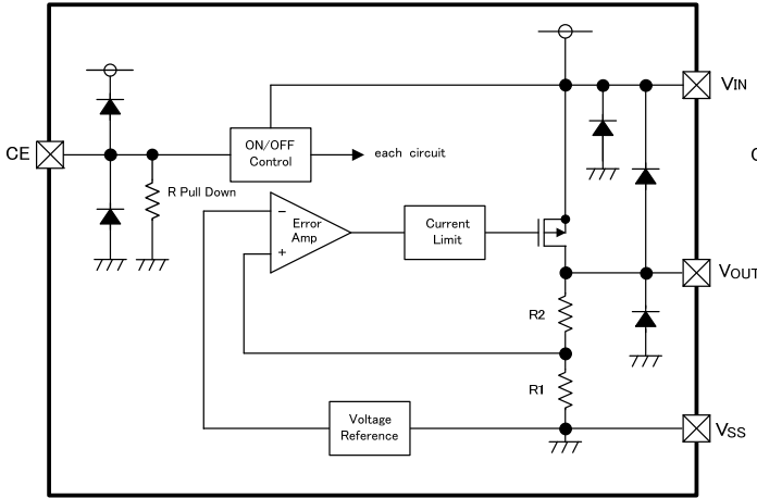
XC6211, XC6219 series Type C, G
