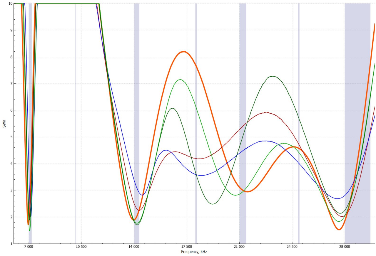
Figure 38: Typical VSWR measurements with closed 17-meter-band link
