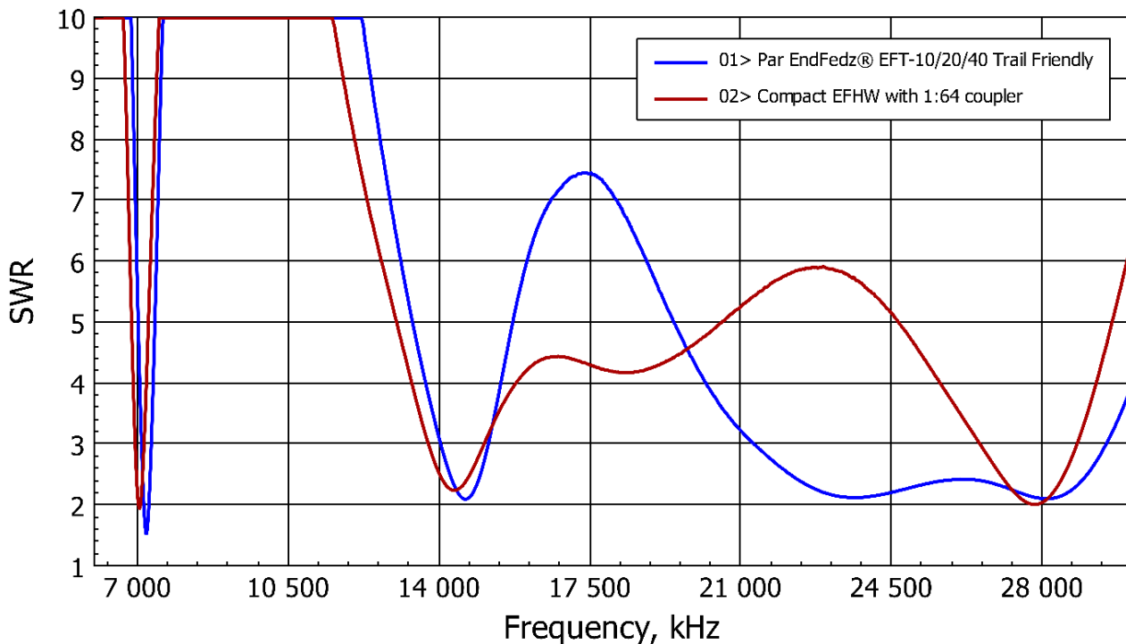
Figure 42: Comparison of a commercial vs. a compact EFHW
