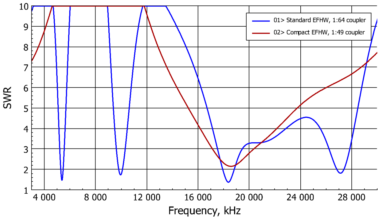
Figure 41: VSWR comparison with enabled 17-meter-band configuration
