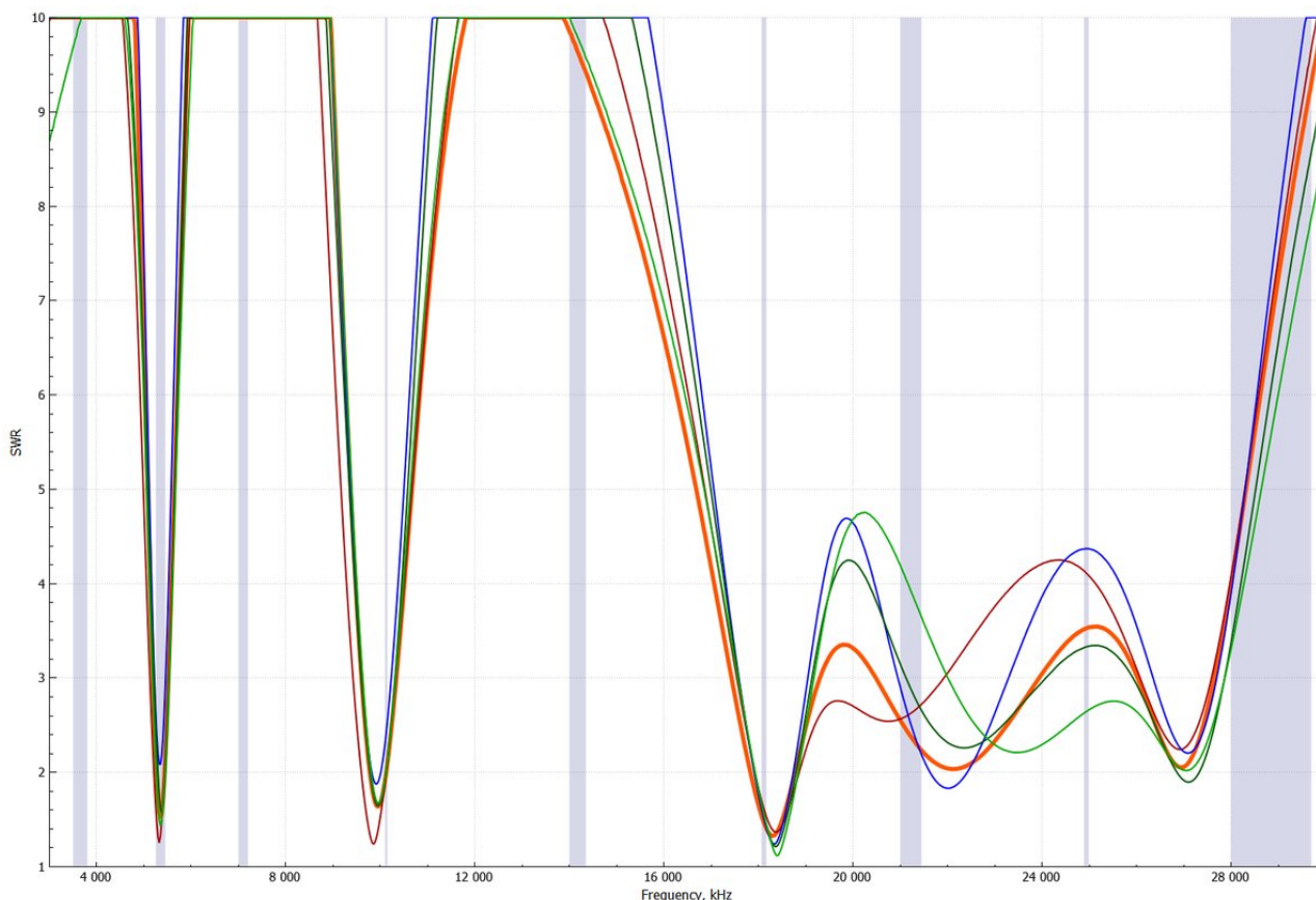
Figure 32: Typical VSWR measurements with enabled loading coil
