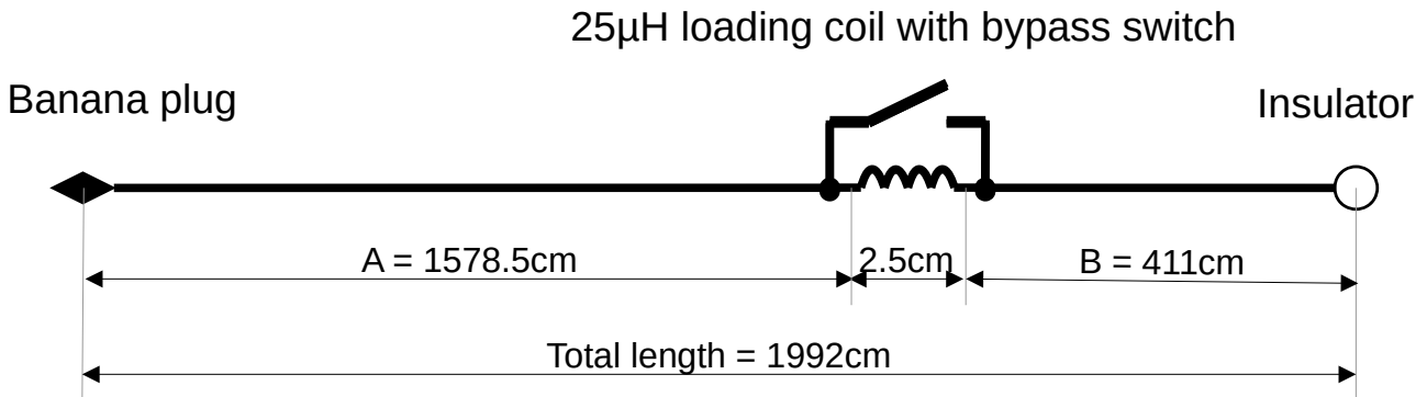
Figure 27: The standard antenna dimensions
