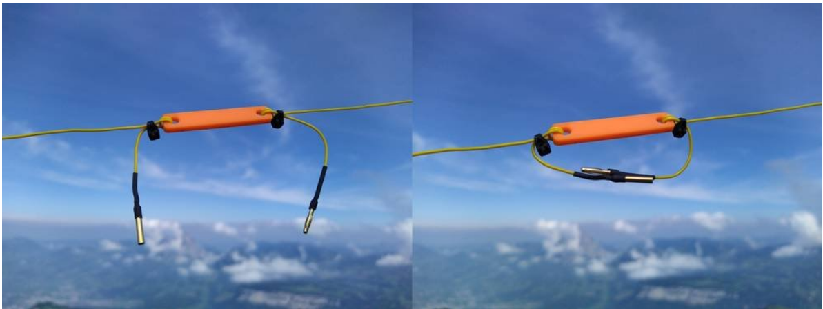
Figure 44: Open link comparison: 200kHz resonance difference at 18MHz
