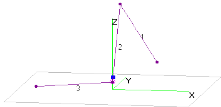
Figure 36: The geometry of the 12m-long inverted-L EFHW antenna setup
