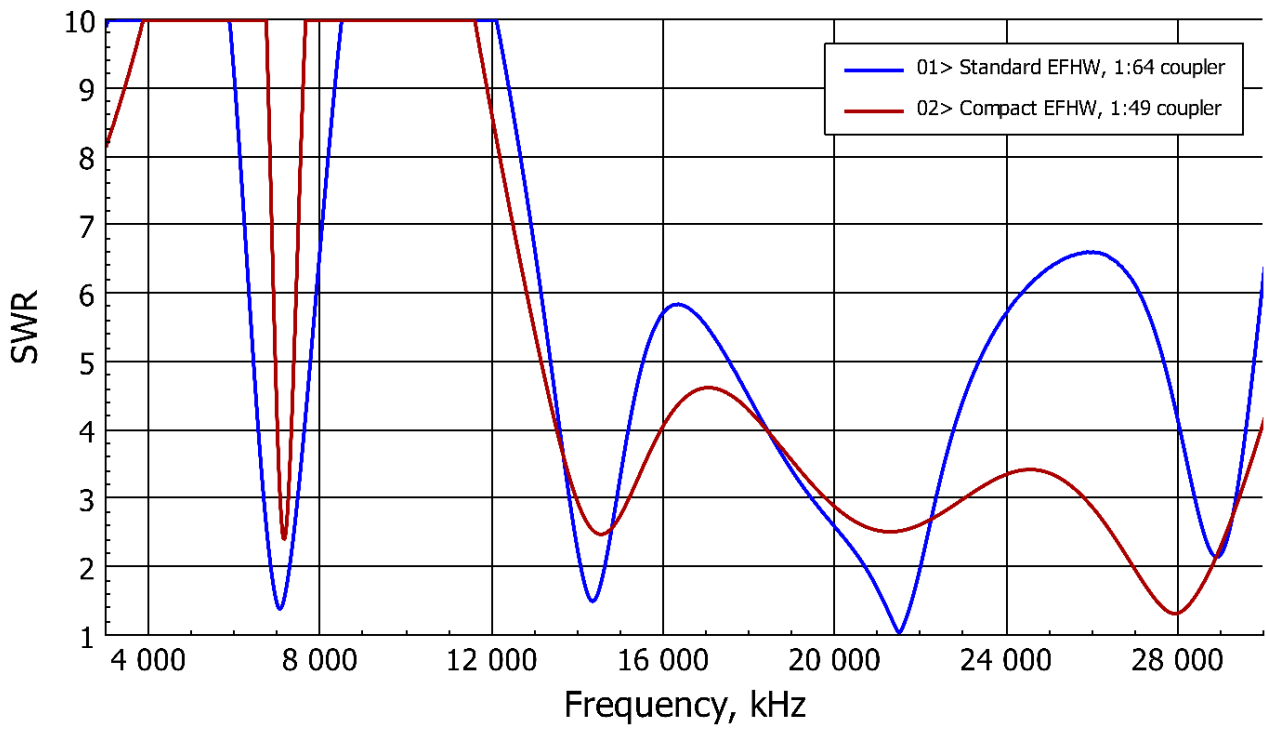
Figure 40: VSWR comparison with standard configuration
