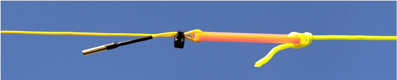
Figure 30: Antenna wire with 2mm gold plated socket, insulator and rope
