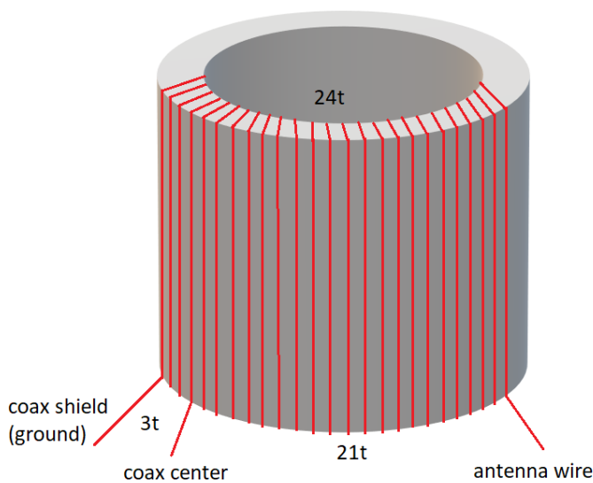
Figure 25: Transformer windings
