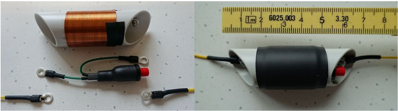
Figure 28: Building the switchable loading coil
