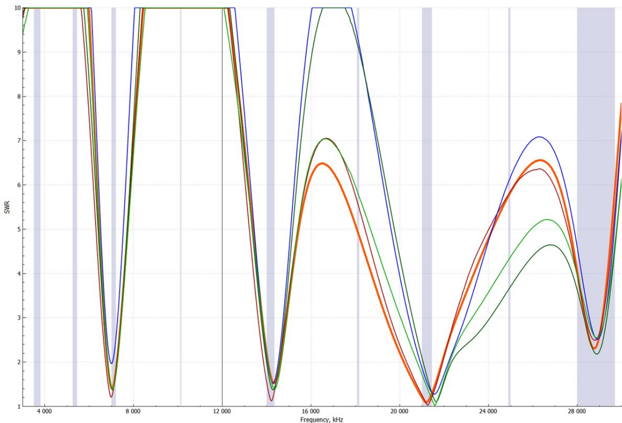
Figure 31: Typical VSWR measurements with bypassed loading coil
