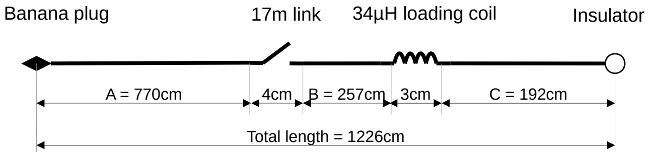
Figure 37: The compact antenna dimensions
