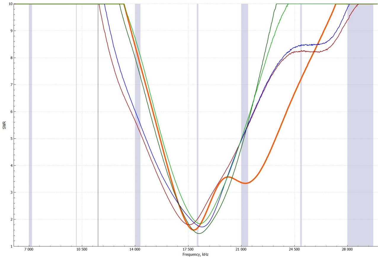
Figure 39: Typical VSWR measurements with open 17-meter-band link
