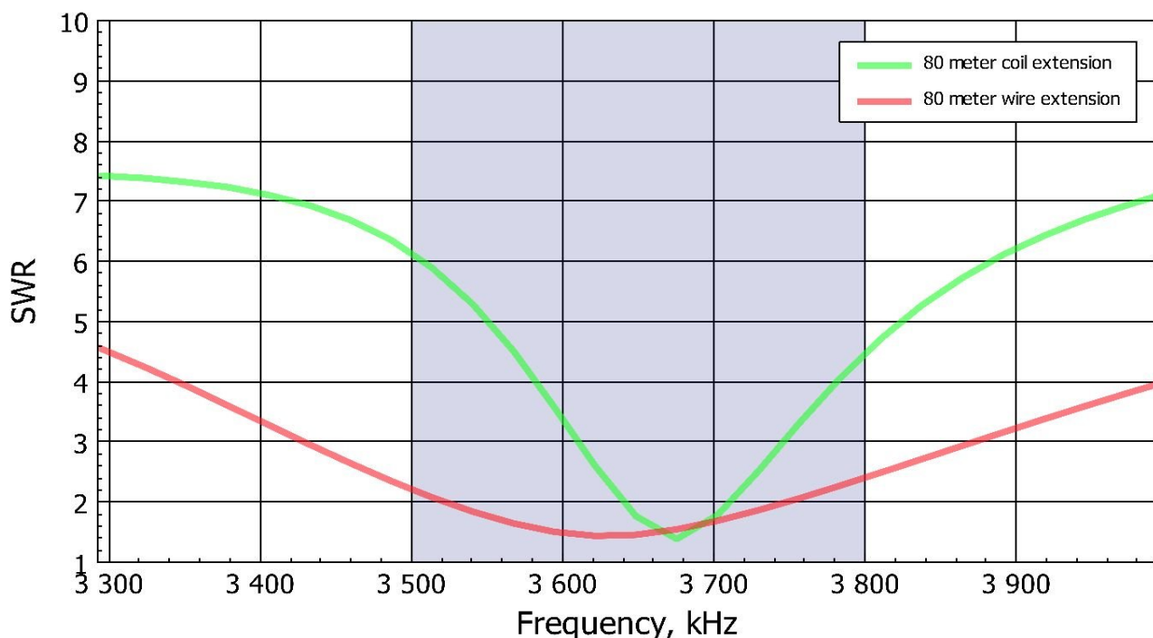
Figure 34: Comparison of the bandwidth of both solutions
