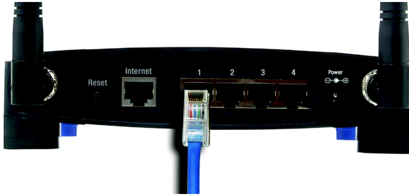
Figure 4-2: Connecting Your Network Devices
