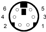
PS2 Mouse (6-pin female)
