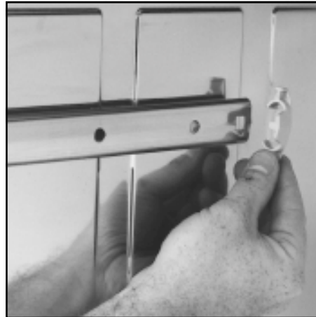
Fig. 5-3 To remove the Rail, disengage the End Cap by applying outward pressure to the Cap's top tab, unclipping it from the Rail. Then slide the Rail out from the Guide Rollers.
