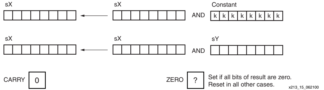
Figure 23: AND Instruction
