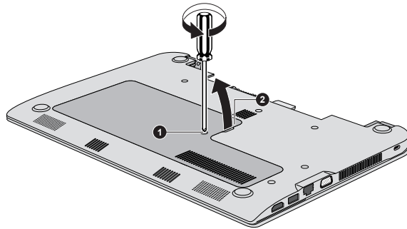
Figure 4-5 Removing the memory module cover
