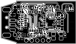
PCB dimensions 46x26mm
