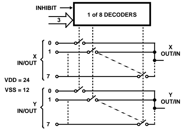
CD4097
