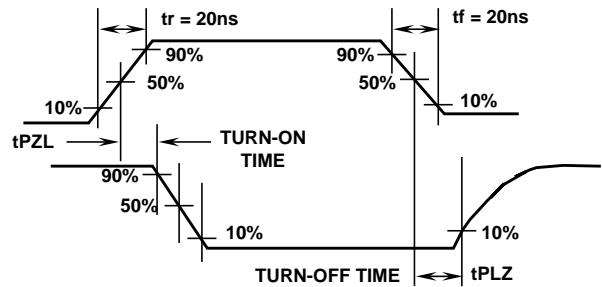
FIGURE 1. WAVEFORM CHANNEL BEING TURNED ON, OFF
