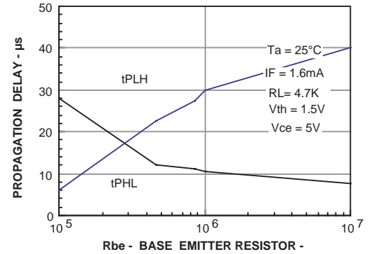
Figure 17. Propagation delay vs. base emitter resistor
