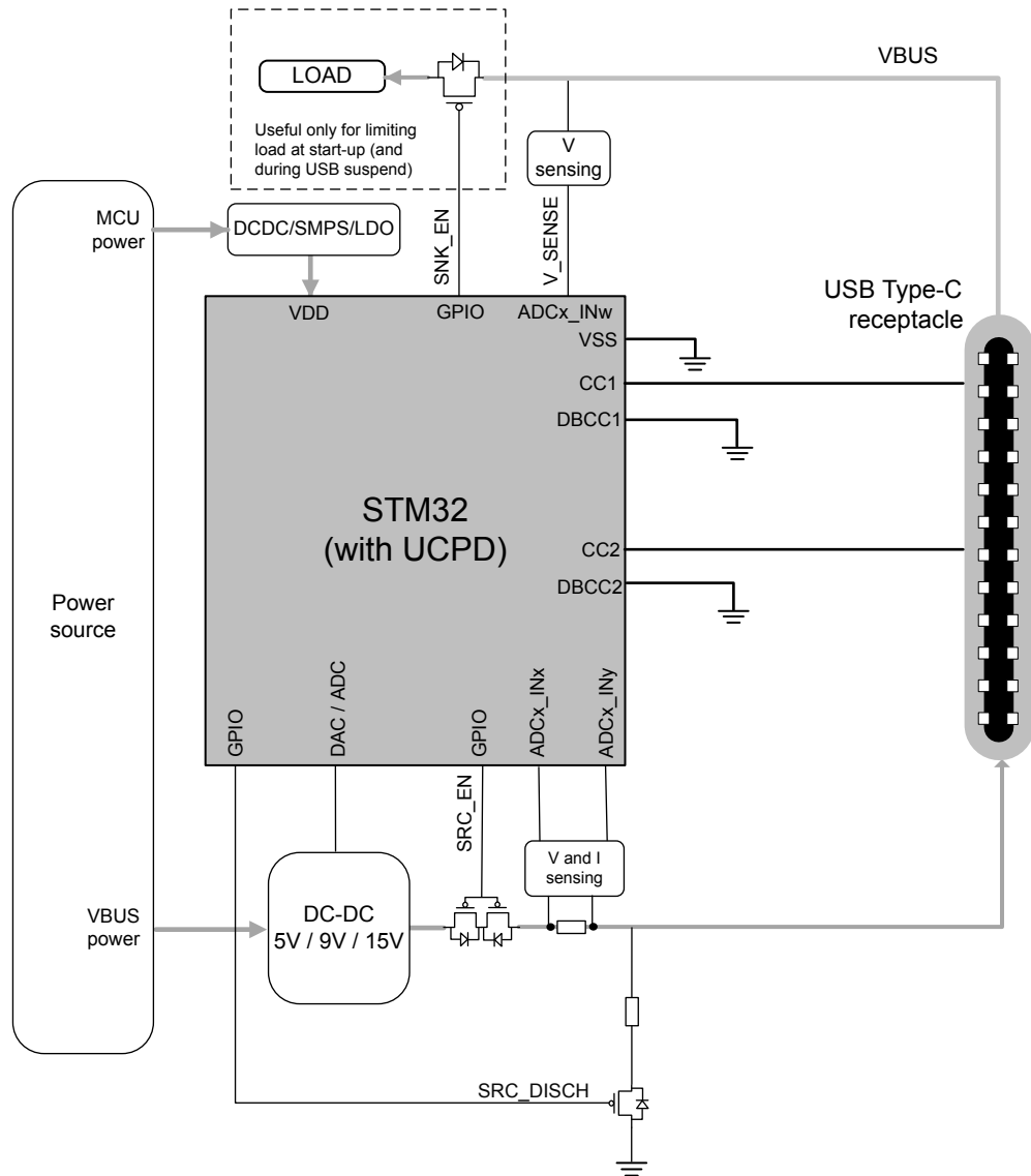
Figure 26. DRP connections
