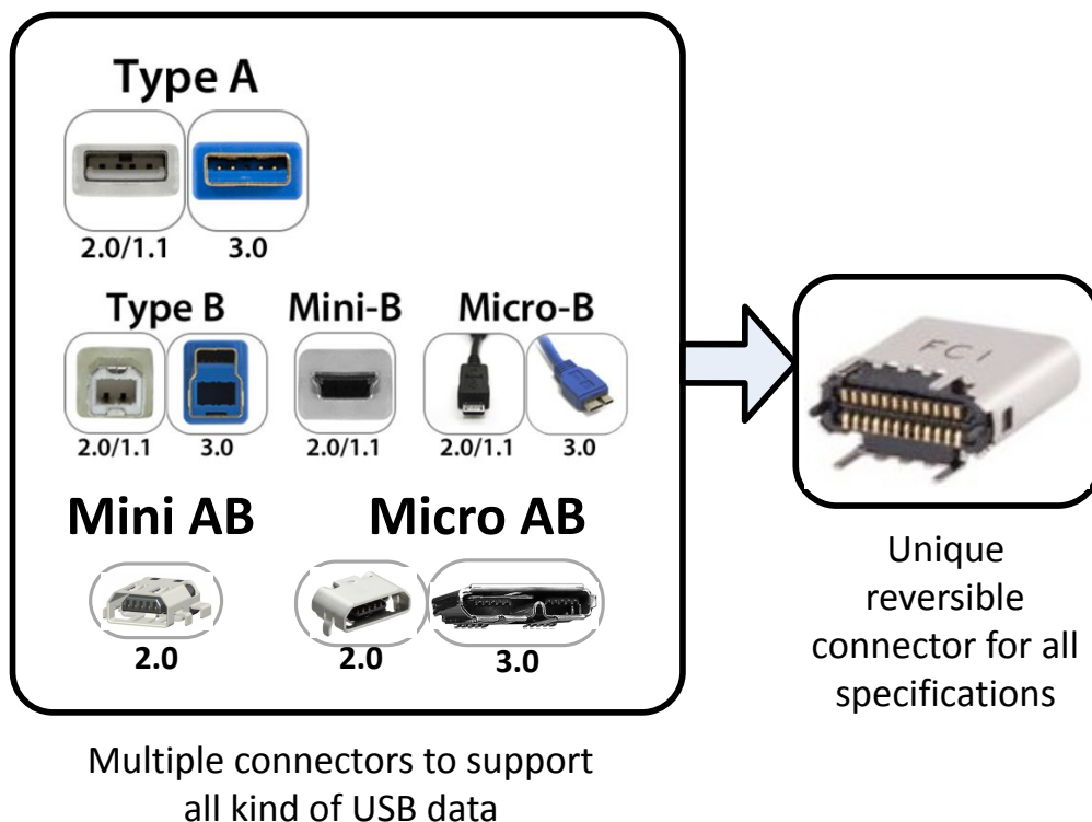
Figure 1. USB connectors
