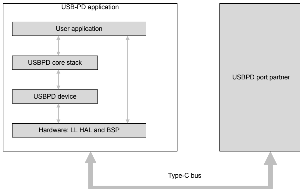
Figure 13. USB-PD stack architecture
