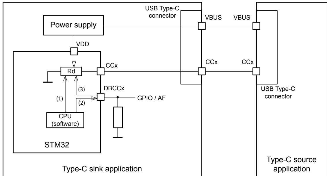
Figure 16. Non-protected sink not supporting Dead battery feature
