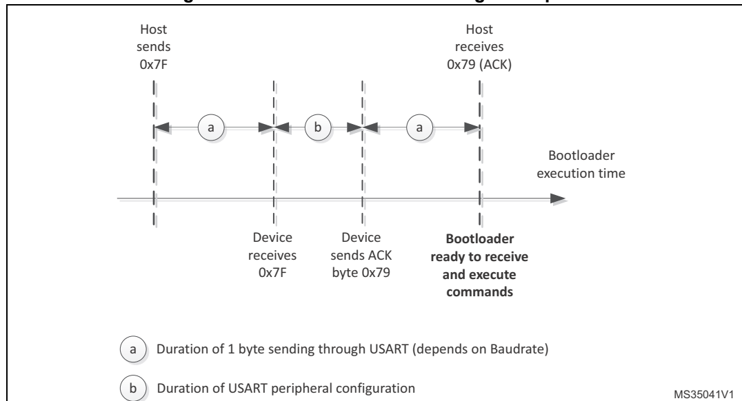
Figure 38. USART connection timing description
