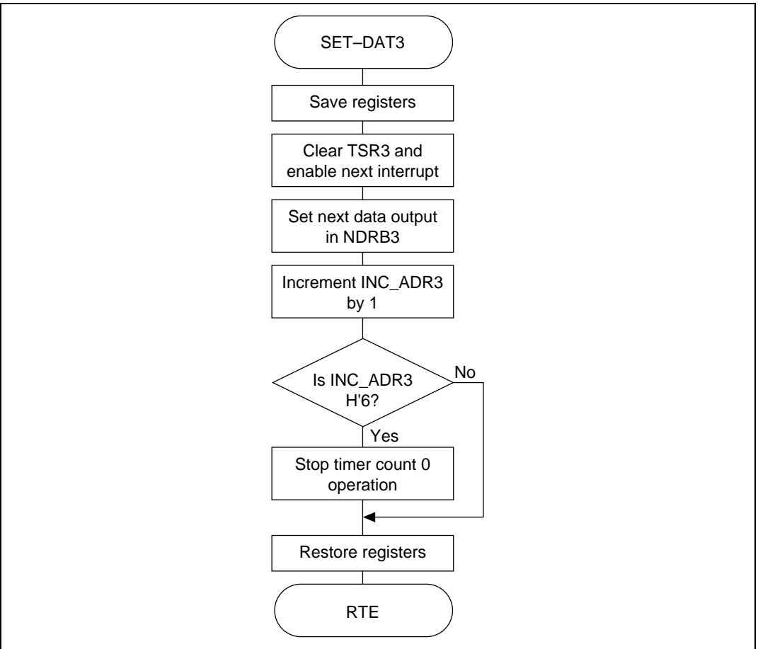
Figure 2.56 SET-DAT3 Flowchart
