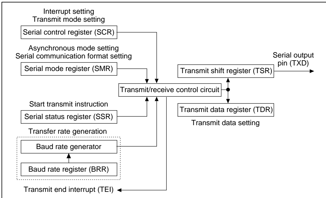
Figure 2.58 Block Diagram of SCI Transmit
