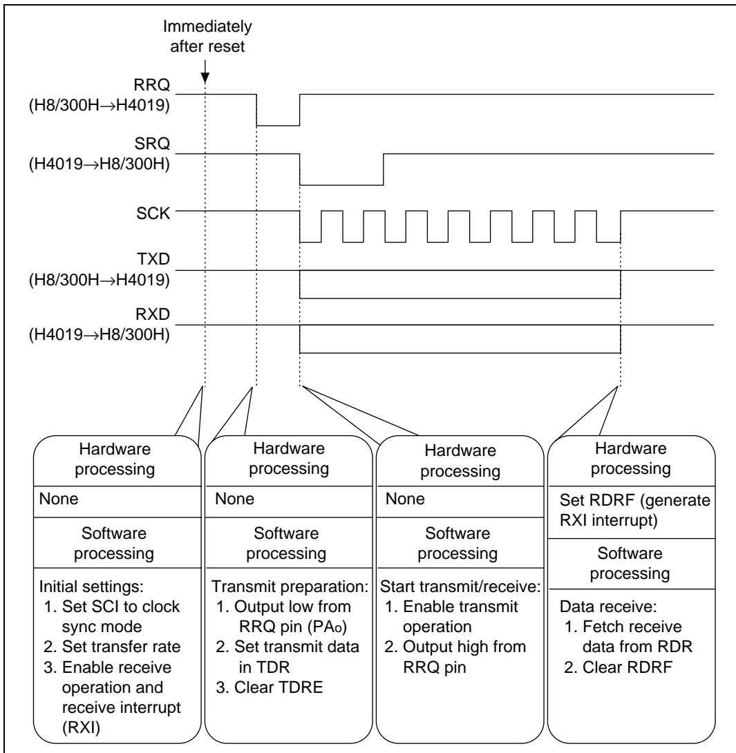
Figure 2.65 Principle of Simultaneous Transmit/Receive Operation
