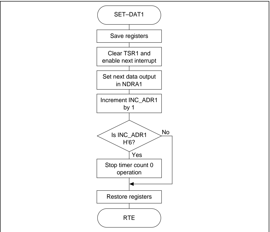
Figure 2.54 SET-DAT1 Flowchart
