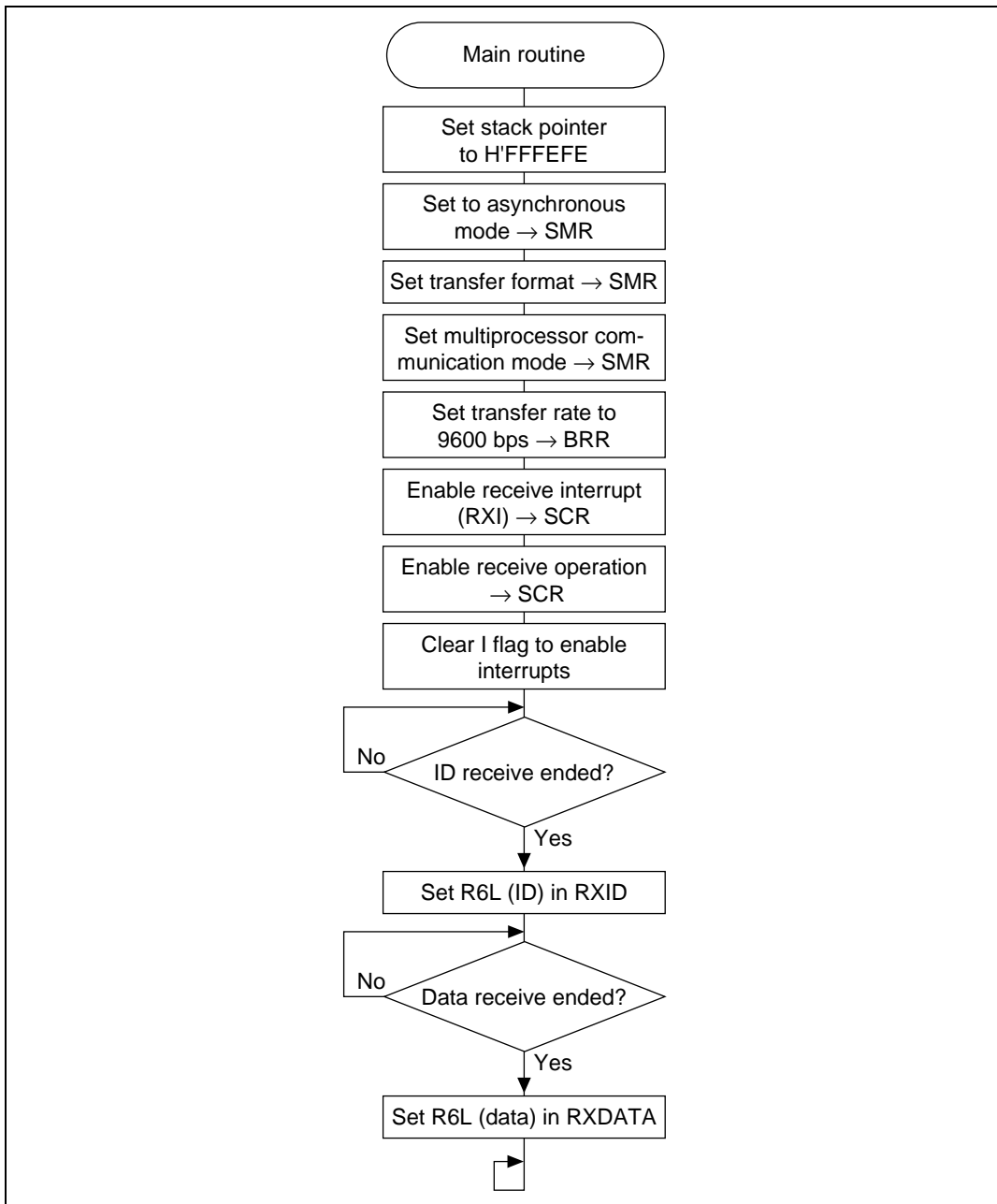
Figure 2.74 Flowchart of Slave Side Software (Main Routine)
