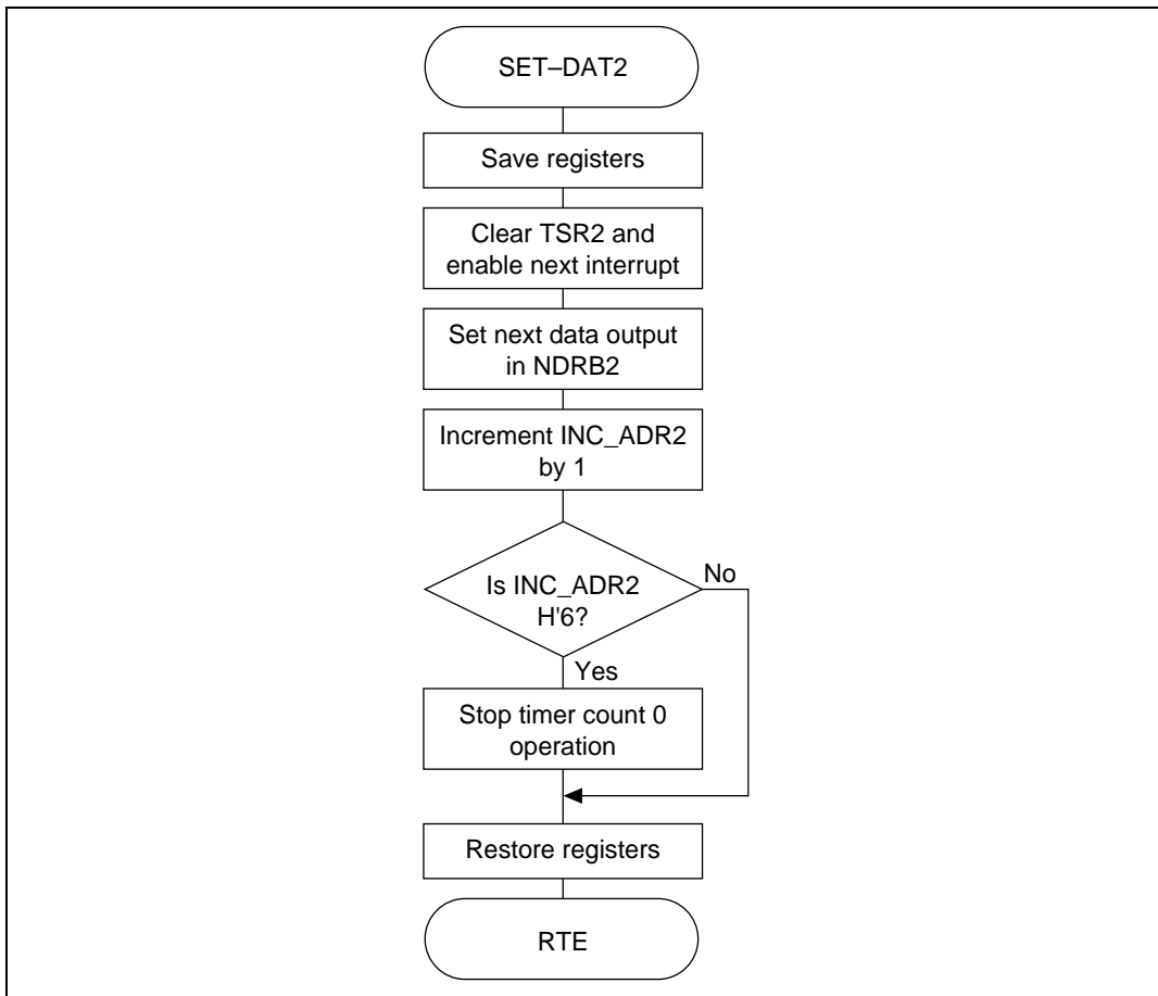
Figure 2.55 SET-DAT2 Flowchart
