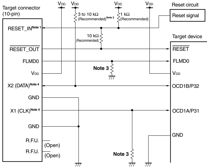
Figure 27-2. Connection Example of QB-78K0MINI or QB-MINI2 and μPD78F0537D (When OCD1A/P31 and OCD1B/P32 Are Used)
