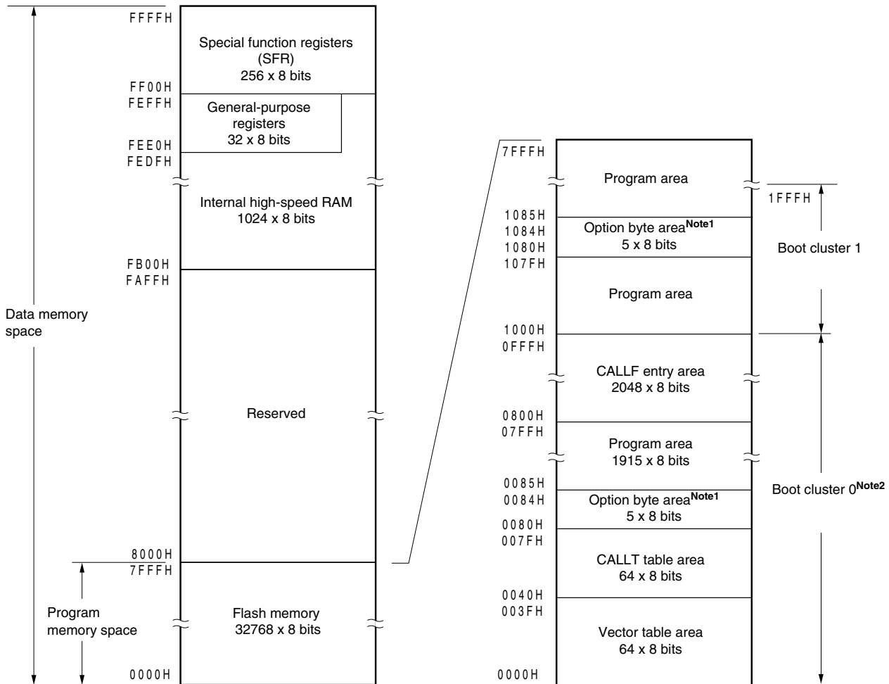
Figure 3-3. Memory Map ( \mu PD78F0533)
