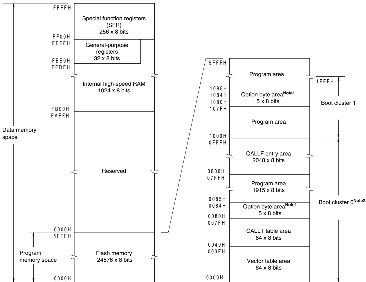
Figure 3-2. Memory Map ( \mu PD78F0532)
