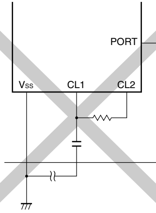
(b) Crossed signal line
