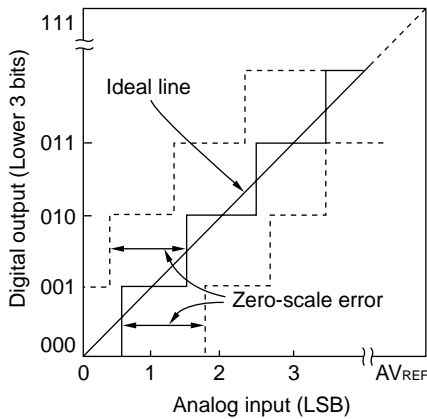
Figure 10-14. Zero-Scale Error
