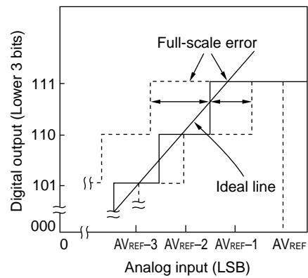
Figure 10-15. Full-Scale Error
