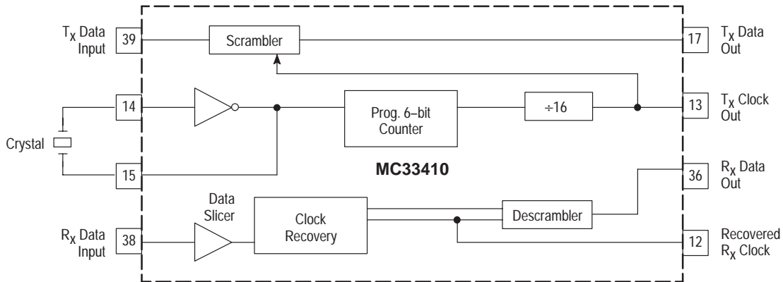
Figure 5. Data Modem Mode Configuration
