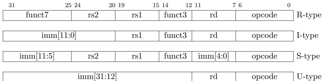
Figure 2.2: RISC-V base instruction formats. Each immediate subfield is labeled with the bit position ( \text{imm}[x] ) in the immediate value being produced, rather than the bit position within the instruction’s immediate field as is usually done.
