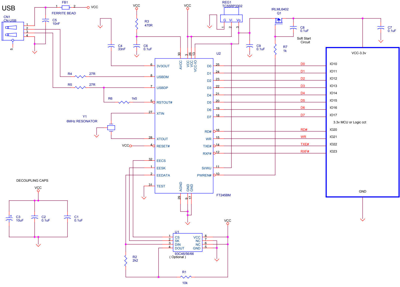
FT245BM 3.3v BUS POWERED EXAMPLE WITH POWER SWITCHING
