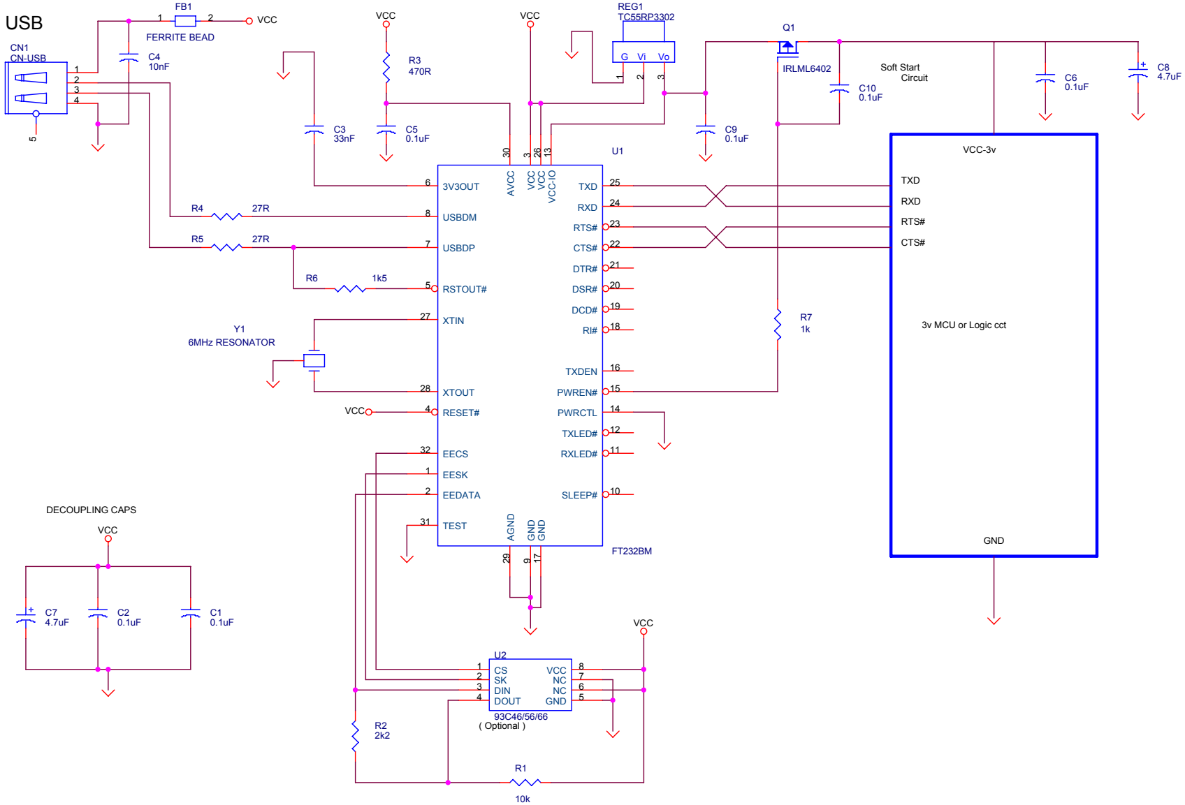
FT232B APPLICATION SCHEMATIC INTERFACING TO 3.3 V LOGIC - BUS POWERED ( <= 250mA ) APPLICATION WITH POWER SWITCHING
