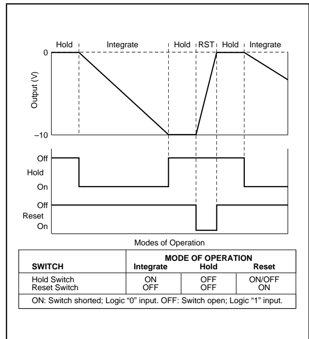
FIGURE 2. Modes of Operation for the ACF2101.
