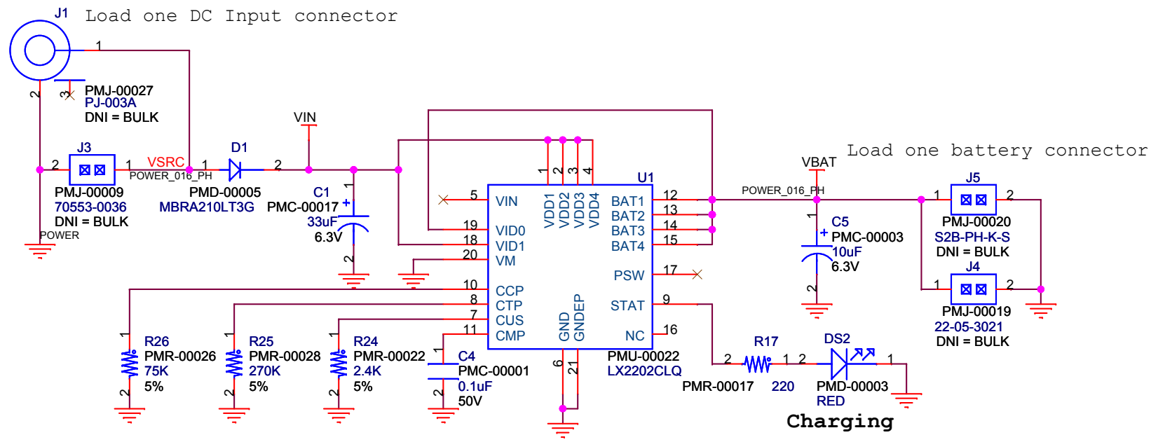
Li/LiPo Charger and Power Selector
