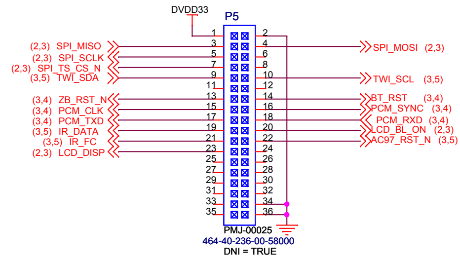
NGW100 Interface
