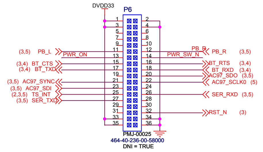
NGW100 Interface
